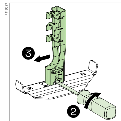
2 Twist the screwdriver to use it as a lever on the click lip until it passes over the bracket's locking lip and 3 pull the adaptor sideways to release it.
