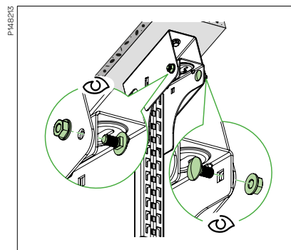
Fix the pendant to the adjustable ceiling plate with 4 bolt sets 22S and align the pendant to the vertical plane before tightening the bolts.
