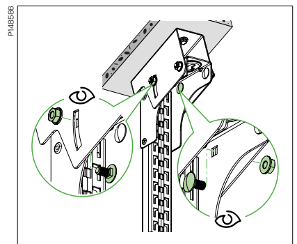
Fix the pendant to the adjustable ceiling plate with 4 bolt sets 22S and align the pendant to the vertical plane before tightening the bolts.
