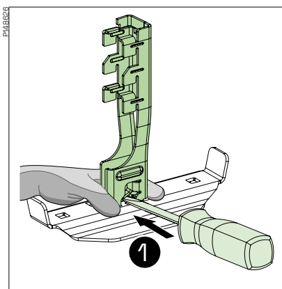
1 Hold the bracket, fit the screwdriver's head between the adaptor lip and the bracket.
