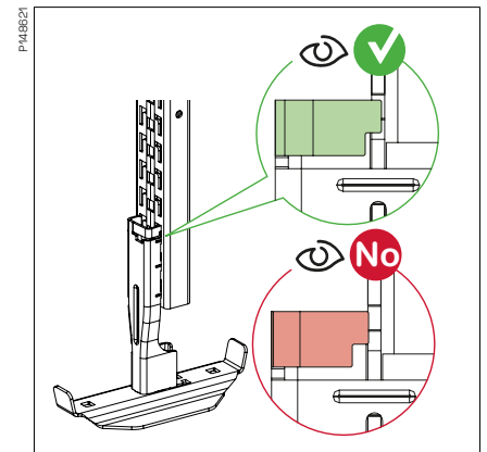
If the adapter needs to be reinstalled, correct the click lip to the initial position and make sure the click lip is locking properly.
