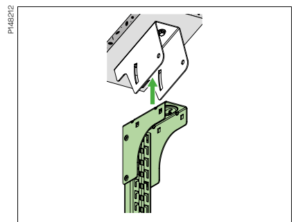
Insert the pendant into the adjustable ceiling plate.
